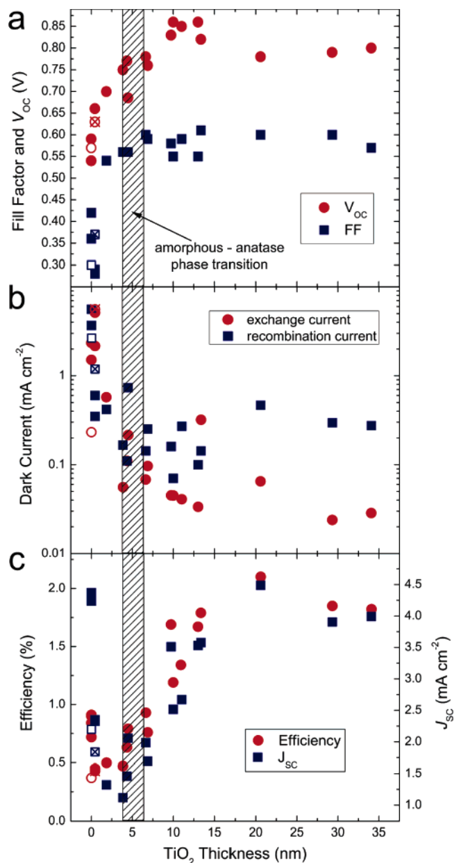
Figure 7. Performance trends for ZnO-TiO 2 core-shell nanowire cells of different shell thickness at a light intensity of 100 mW cm -2 . (a) V_{oc} and fill factor. (b) Dark anodic exchange current and cathodic recombination current on a logarithmic scale. (c) J_{sc} and cell efficiency. Filled symbols: Uncoated ZnO nanowire cells sensitized in dye for 1 h (standard cells) and core-shell cells sensitized for 12 h. Open symbols: An uncoated ZnO nanowire cell sensitized for 1 h. Crossed symbols: A core-shell cell sensitized for 1 h. The hatched region indicates the onset of the phase transition from amorphous to anatase TiO 2 .
